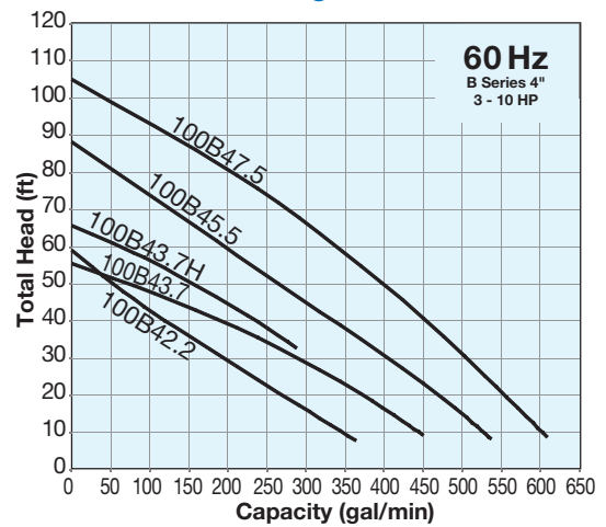
With TO /TOS Guide Rail System
